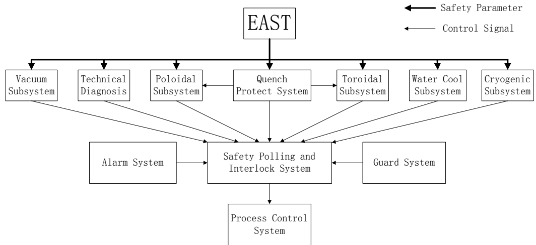
Fig.3. The structure of EAST Safety & Protect System
