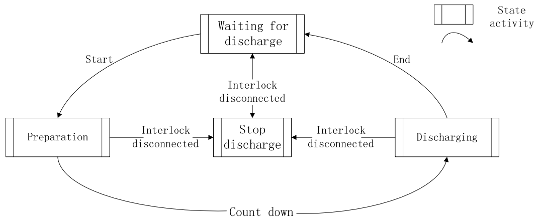
Fig.4. EAST process control logical
