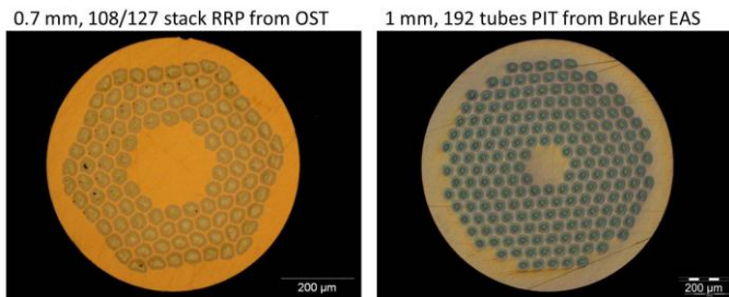
Fig. 3 Nb 3 Sn layouts from leading ITD Nb 3 Sn manufacturers.
