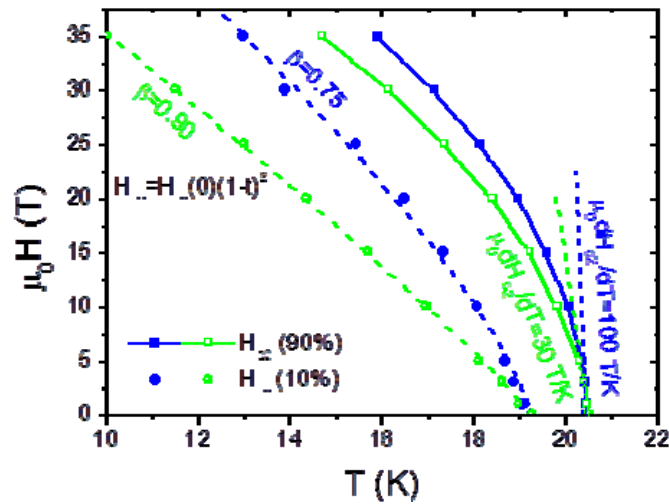
Fig. 2 Upper critical field and irreversibility line as derived from resistive transitions in parallel and perpendicular direction. The slope of H_{c2} close to T_c is also shown. H_{irr} are fitted by power law.
