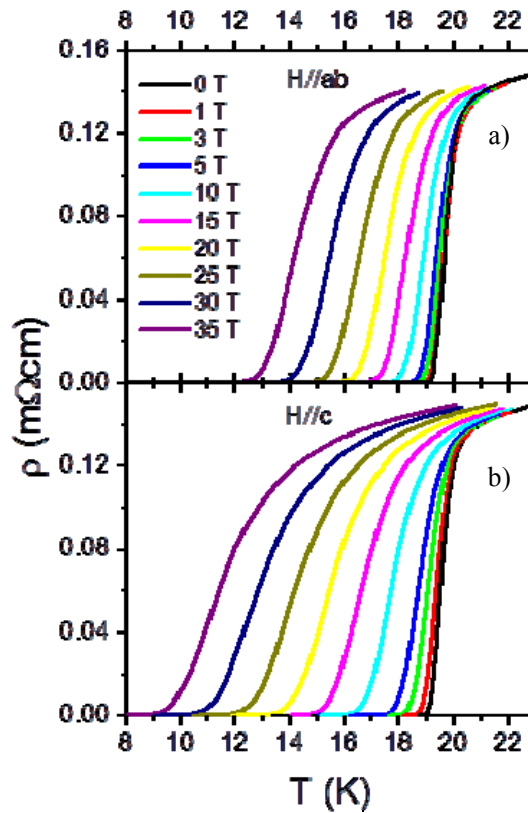
Fig. 1 Resistive transitions in magnetic field up to 35 T, applied parallel (a) and perpendicular (b) to the ab plane.
