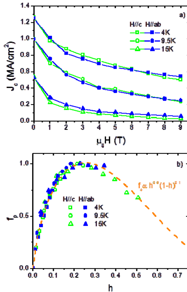
Fig. 4 a) Critical current density as a function of magnetic field at selected temperature and b) the relative normalized pinning force as a function of the reduced magnetic field H/H_{irr} . The curves are fitted by the Dew-Hughes relation.
