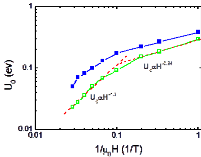
Fig. 3 Vortex motion activation energy as a function of the inverse of the field in parallel and perpendicular configuration as extracted from the Arrhenius plot.
