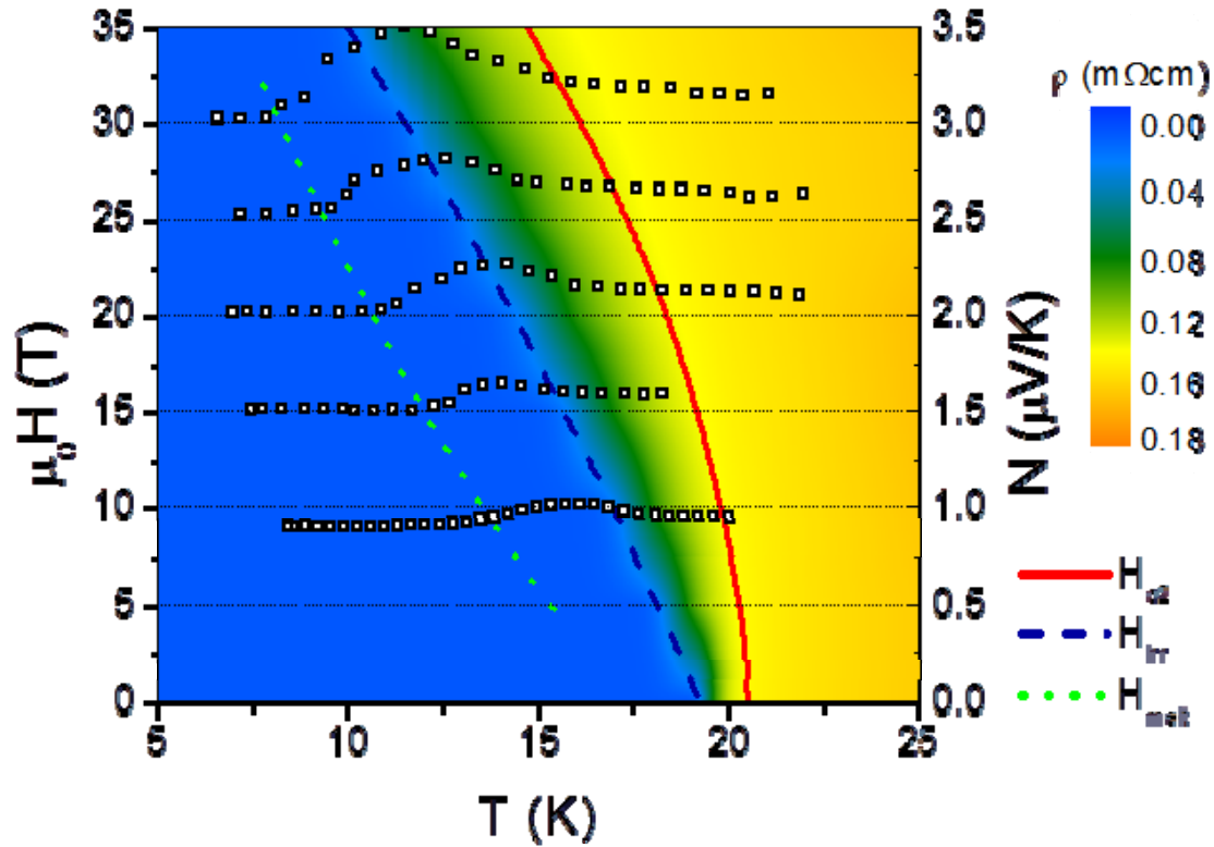
Fig. 6 Fe(Se,Te) Vortex phase diagram combined from resistivity (2D plot) H_{c2} and H_{irr} (left scale) and offsetted (see text) Nernst effect (right scale). All quantities are measured with the magnetic field applied perpendicular to the ab planes.
